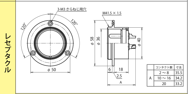
NCS-40 ■ -R
