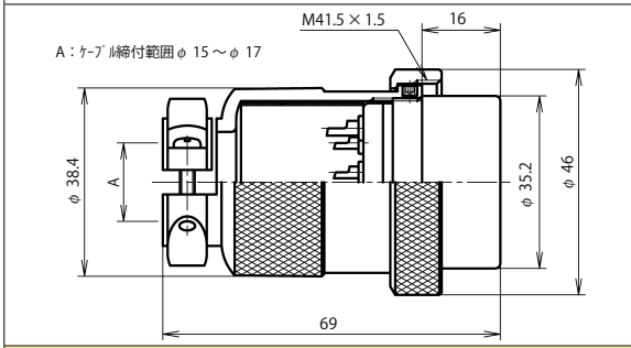
NCS-40 ■ -P
