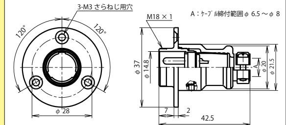
NCS-16 ■ -Ad(F)-CH
