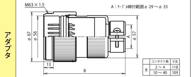
NCS-60 ■ -Ad
