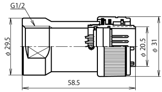
NR-24 ■ -GPM1/2 (注)
