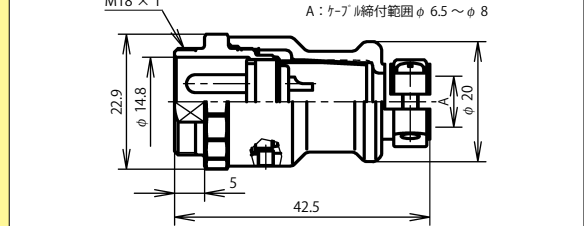
NCS-16 ■ -Ad-CH
