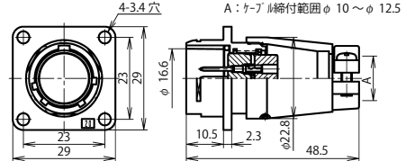
NR-20 ■ -Ad(F)M
