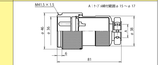
NCS-40 ■ -Ad
